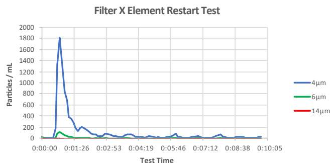
Figure 8: Filter X DFE Restart Test
