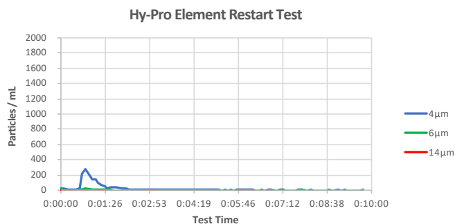
Figure 9: Donaldson Hy-Pro DFE Restart Test
