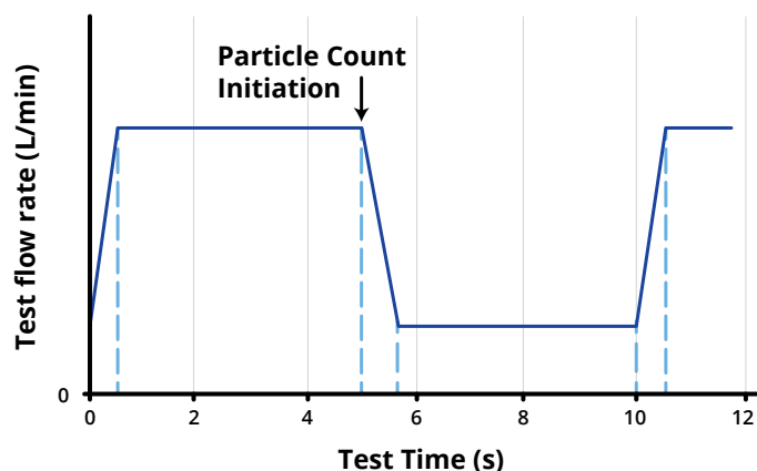
Figure 5: ISO23369 Flow Cycle
